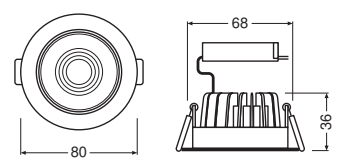
707993_LEDVANCE Spot LED adjust 4W and 6W
